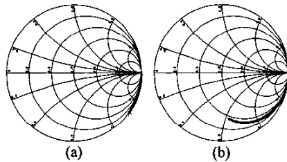
Fig. 2. Electrical lengths (S21 phases) of two microstrip lines up to 10GHz over (a) the de-embedded plane "A" in Fig. 1 (a) and (b) the de-embedded plane "B" in Fig. 1 (b).
