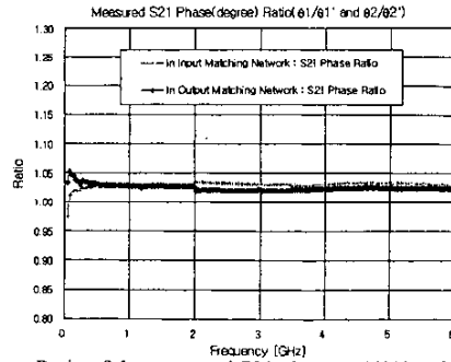
Fig. 5. Ratio of the measured S21 phases, \theta_1/\theta_1' and \theta_2/\theta_2' .
