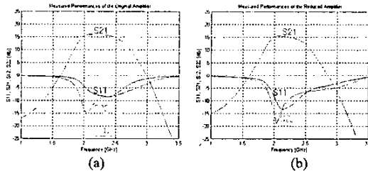
Fig. 6. Measured performances of the (a) original and (b) reduced amplifier.
