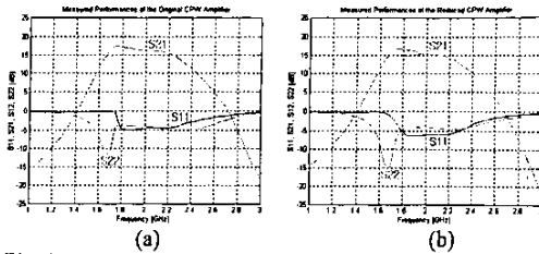
Fig. 9. Measured performances of the (a) original and (b) reduced CPW amplifiers
